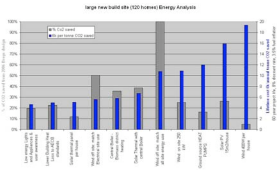
Figure 1. Graph showing cost per tonne of carbon saved per year. Micro wind was the most expensive measure with the lowest yield 10 Low energy appliances and improvements to the building shell were the cheapest. Peter Warm and Nick Grant for NBT Consult.
