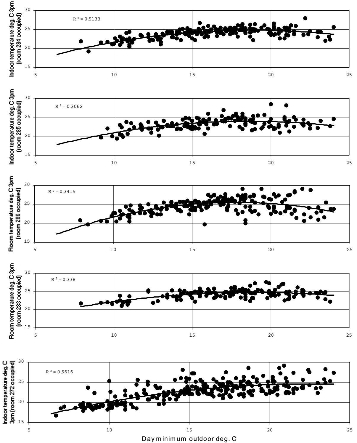
Figure 12. Day by day temperature variations in five typical rooms when occupied.
