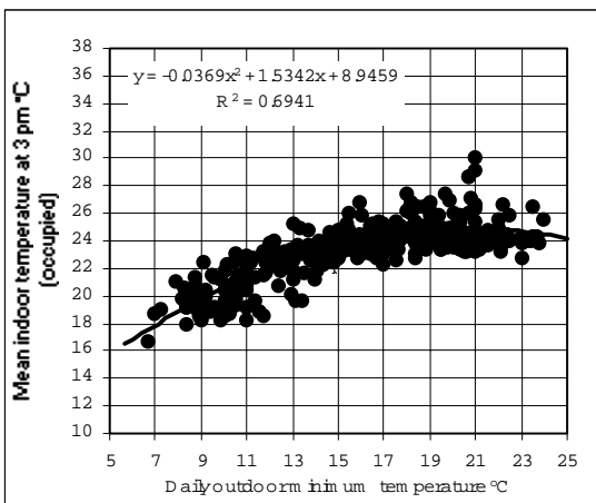
(iii) Mean indoor temperatures in occupied rooms at 3 pm.
