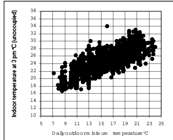
(ii) Indoor temperatures in unoccupied rooms at 3 pm.
