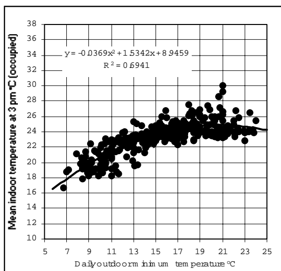
(i) Mean indoor temperature at 3 pm. Binomial regression with daily outdoor minimum temperature as independent variable.
