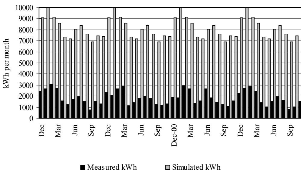
Figure 4. Month by month energy consumption of the supplementary cooling/heating system from December 1997 to November 2001 compared with estimated consumption for a conventional air conditioning system for the same spaces with fixed windows.
