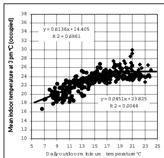
(ii) Mean indoor temperature at 3 pm. Linear regressions with daily outdoor minimum temperature as independent variable.
