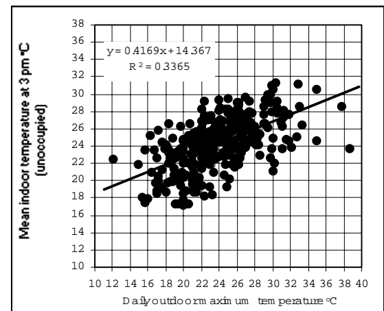
(vi) Mean indoor temperatures in unoccupied rooms at 3 pm.
