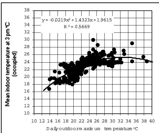
(v) Mean indoor temperatures in occupied rooms at 3 pm.
