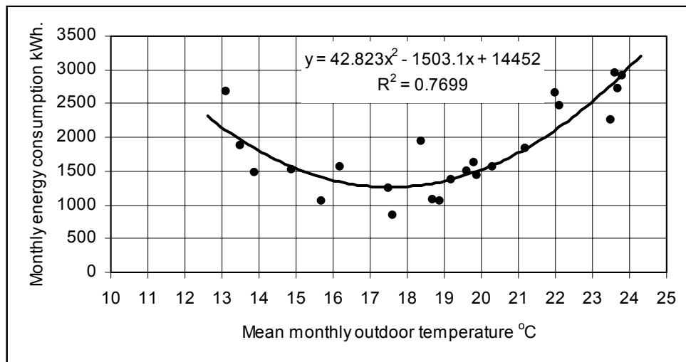
Figure 5. Relationship between monthly energy consumption and mean monthly outdoor temperature.
