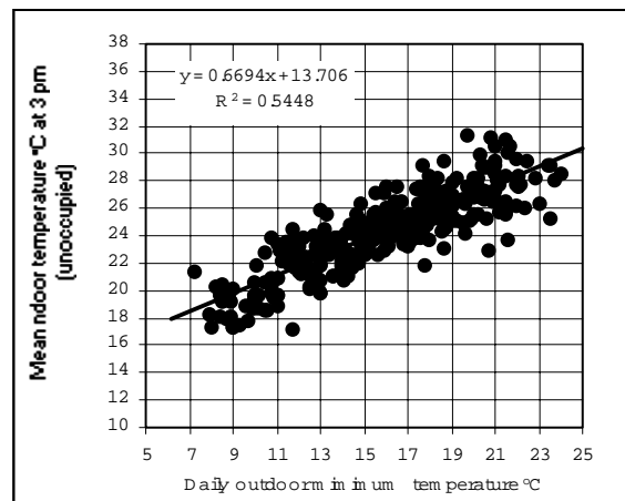
(iv) Mean indoor temperatures in unoccupied rooms at 3 pm.
