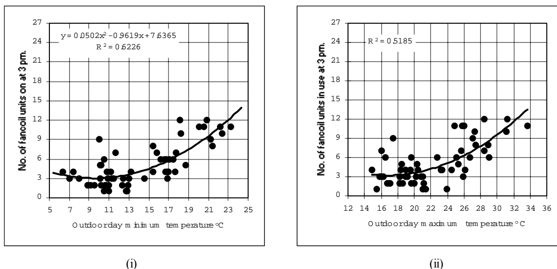
Figure 13. Number of fan coil units in use at 3 pm with outdoor temperature as independent variable.
