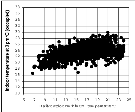
(i) Indoor temperatures in occupied rooms at 3 pm.
