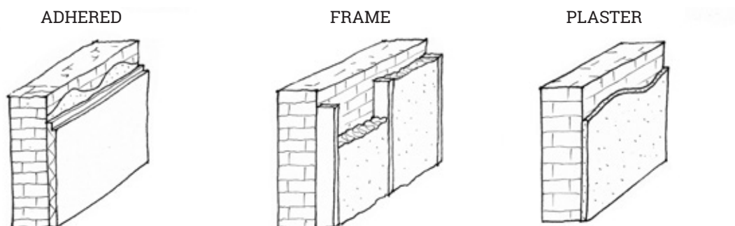
Figure 4: internal wall insulation options. Image © Kaat Janssens
